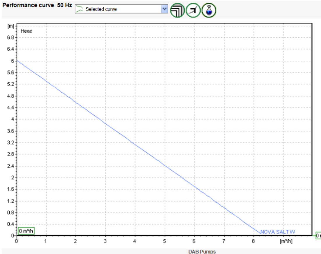
Performance curve 50 Hz
